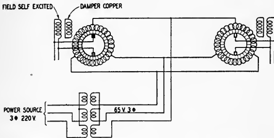
FIG. 2. Method of operation requiring no change in the motors.
